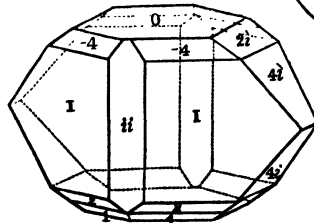
Bergen Hill.
